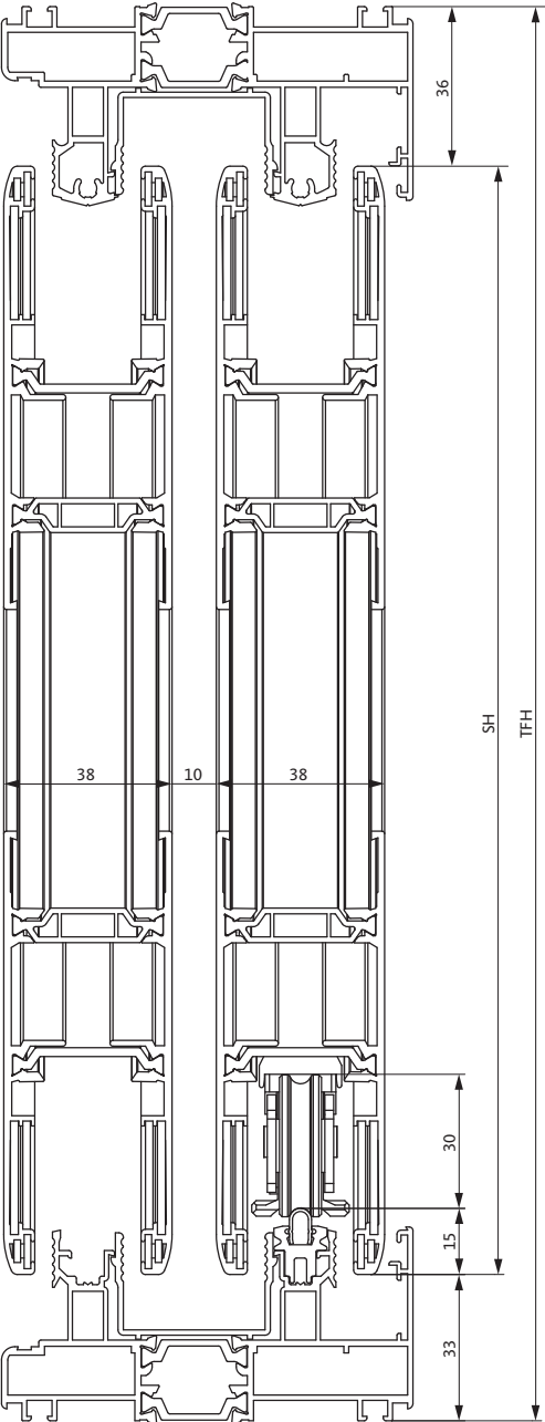
SH = sash height / TFH = total frame height
