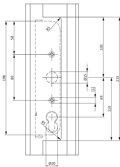
Drilling-hole pattern for turn handle
