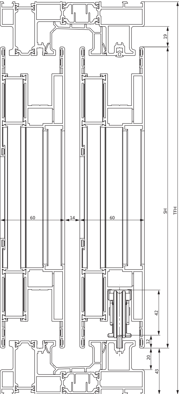
SH = sash height / TFH = total frame height
