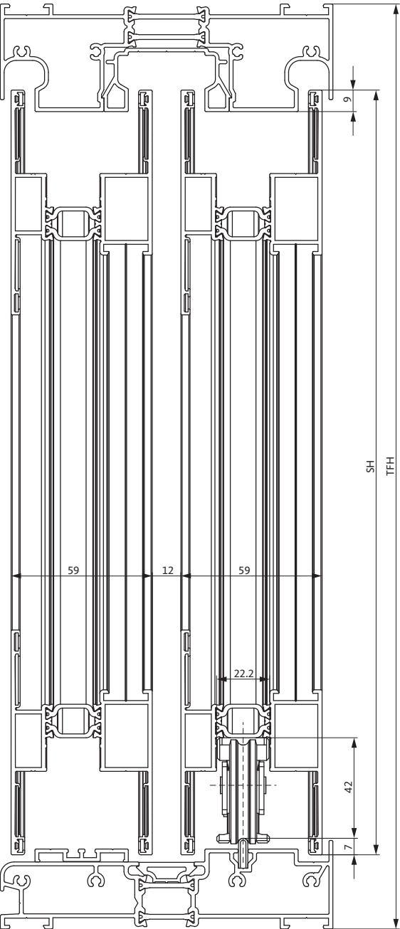
SH = sash height / TFH = total frame height
