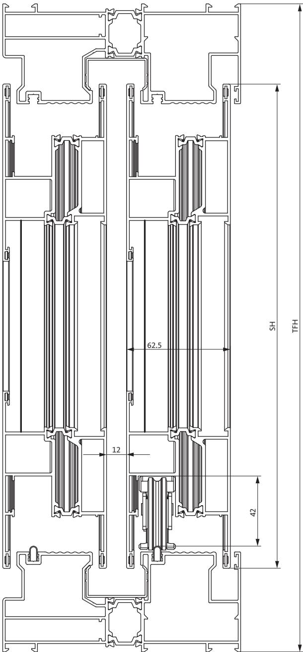
SH = sash height / TFH = total frame height
